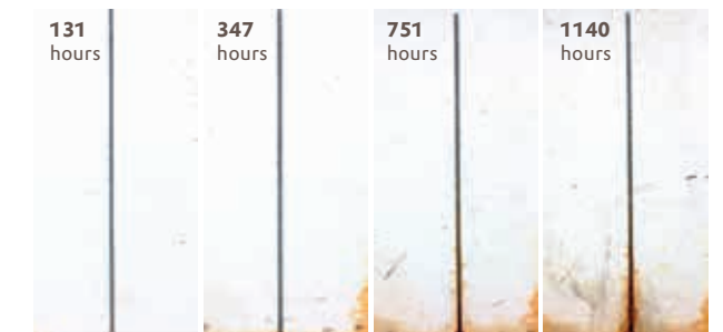
A high zinc content formulation (Table 2) based on Dynasylan® SIVO 140 was applied on shot blasted steel (surface roughness ELK 0.12 – 0.25 mm). Dry film thickness: ~ 70 µm. The zinc-dust paint was overcoated with a water-borne epoxy coating (70 – 80 µm dry film thickness) and placed in a chamber with neutral salt spray fog.
